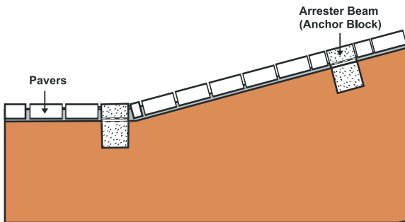
Arrestor Beam (Anchor Block) can be between 25 to 60ft depending on the degree of slope
