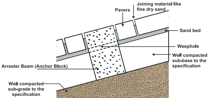
Picture shows how an Arrestor Beam or Block is provided to prevent lateral movement
