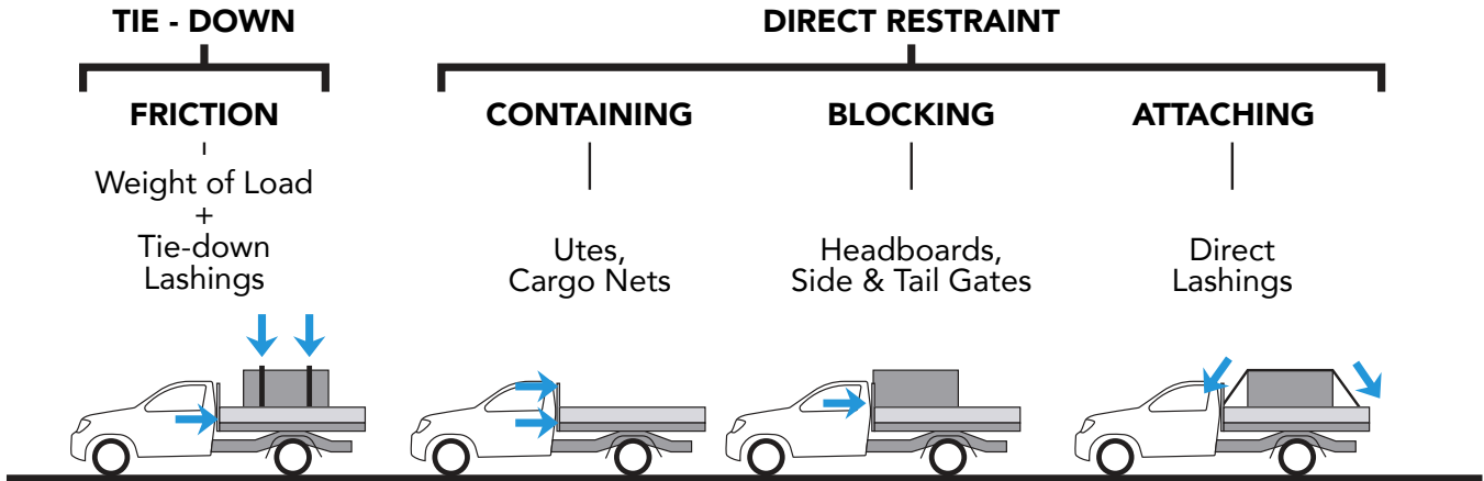
Figure 3: Tie-down and Direct Restraint (Load Restraint Guide - 2018: Page 13)
